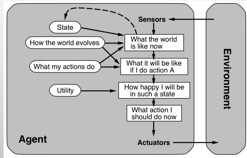
Utility-based Agent
